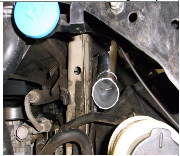
40. Install hdi intercooler cold pipe thru the back of the head light step3
