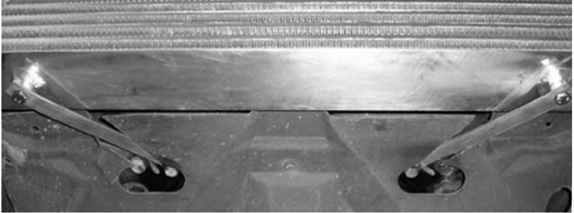
Install the bottom intercooler bracket
